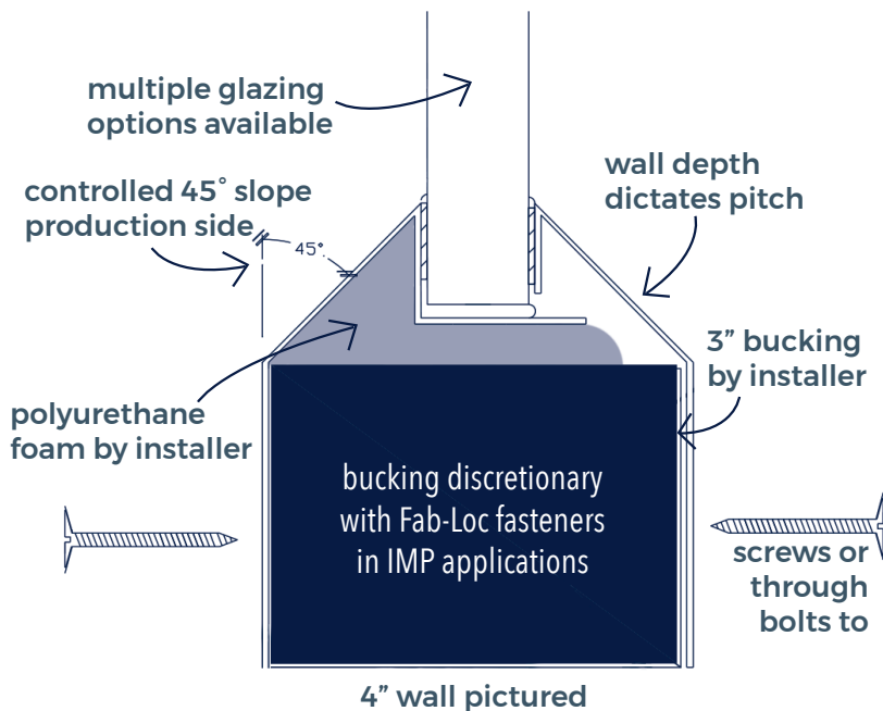
SILL DETAIL
